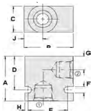
2 Way Housings
