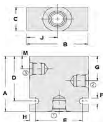
3 Way Housings
