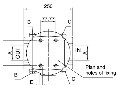
Flange dimensions
