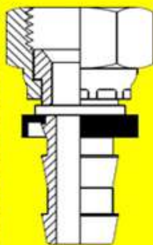
JIC Female
