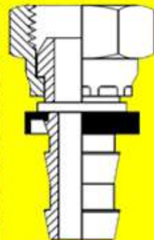
BSPP Female
