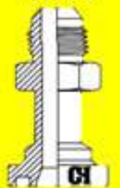
JIC MALE
