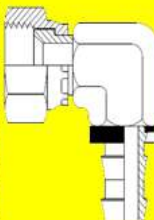
JIC 90° Elbow
