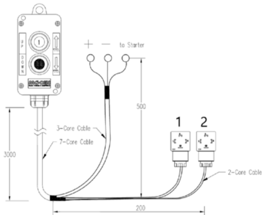
KCB22-03-DIN
